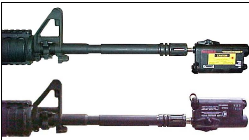
Figure 8-3. Borelight in the START POINT position.
